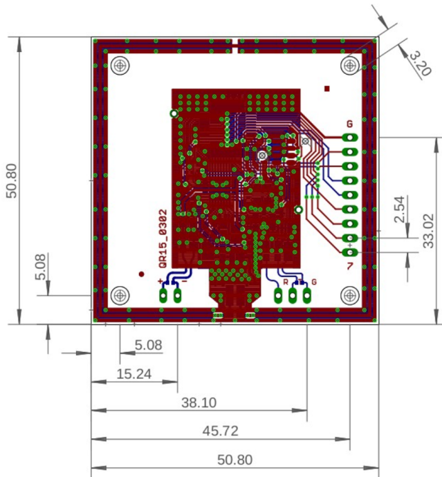
Figure 3. Mechanical Dimensions QR15 v2
