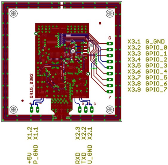
Figure 2. QR15 Pin Positions and Naming (top view)
