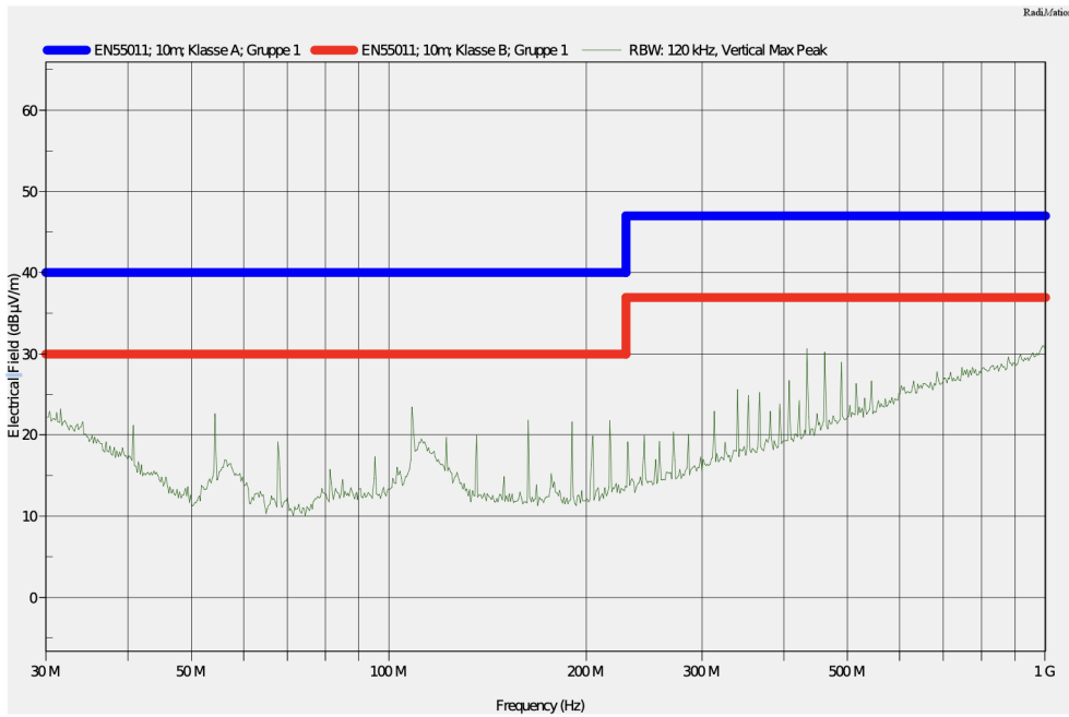
Figure 4. Radiated Emissions of QR15 RFID engine on metraTec evaluation board at full output power (200mW), 2250 mm 2 antenna area
